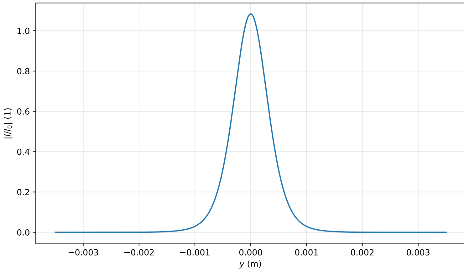
Intensity profile I(x=0, y, z=2.070)/I_0 , P_{in}=0.7P_{cr} , artificial time
